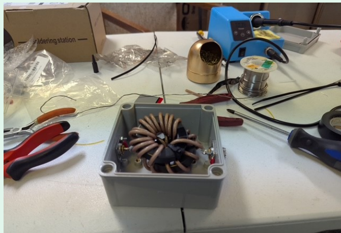
Internals of the choke
